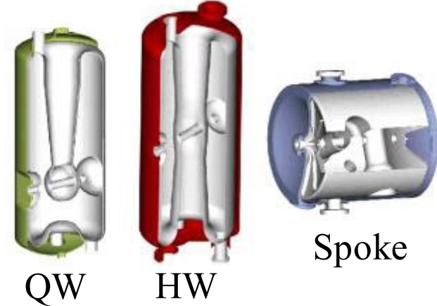
ANL cavities for RIA
