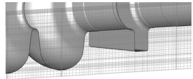
Hexahedral mesh
