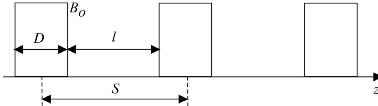
Periodic structure of focusing solenoids.
