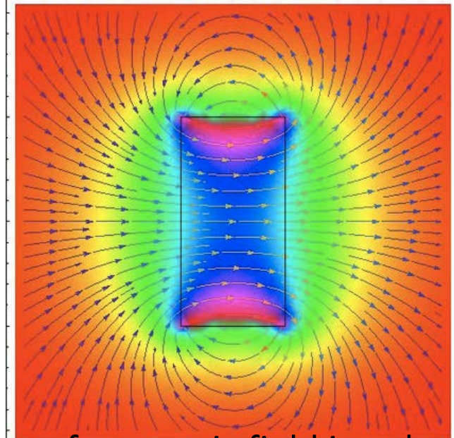
FNAL Solenoids
